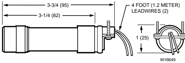
Fig. 4. Installation dimensions of C7927A1016 (U.S.A. version) in in. (mm).
