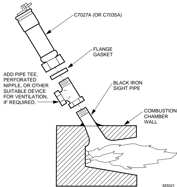
Fig. 7. Mounting a C7027A or C7927A on a combustion chamber (viewed from above). C7035A mounting is similar.
