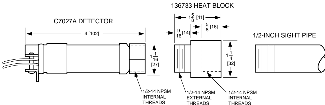
Fig. 8. Mounting dimensions of 136733 Heat Block in. (mm).
