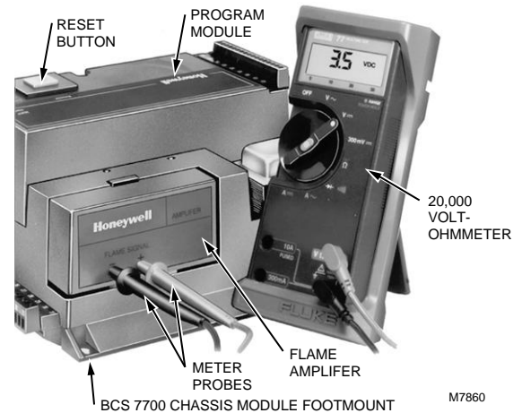
Fig. 13. Measuring the BCS 7700 flame signal voltage.
