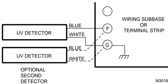
Fig. 10. Wiring C7027A, C7927A, C7035A, and C7044A flame detectors in parallel.
