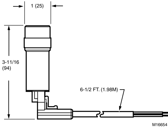
Fig. 5. Installation dimensions of C7927A1008 (European version) in in. (mm).
