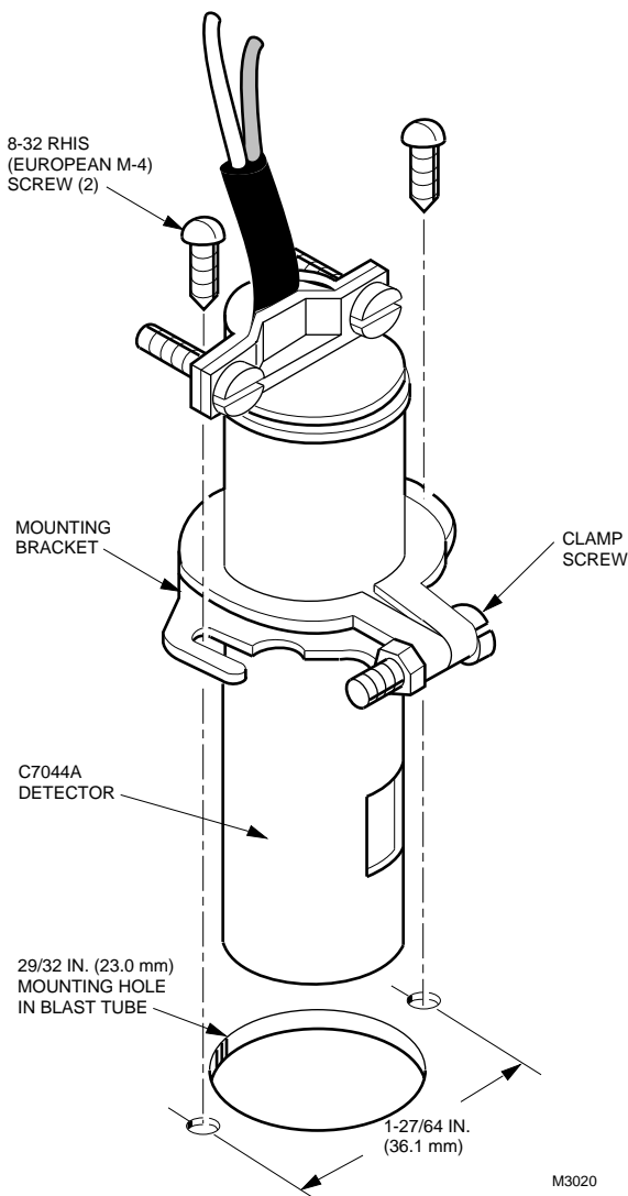
Fig. 9. Mounting C7044A Detector on blast tube.
