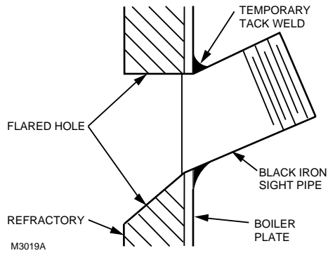
Fig. 6. Mounting sight pipe.
